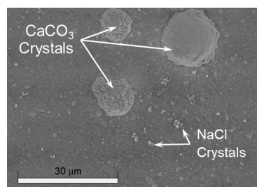
Fig. 2. SEM showed the CaCO 3 and NaCl crystals growth on the membrane; the identities of these crystals were verified by SEM-EDX.
