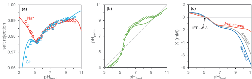
Fig. 1. Experiments (markers) and theory (lines) results illustrating effect of feed pH on (a) rejection of Na^+ (red circles and line), and Cl^- (blue triangles and line), (b) permeate pH (green boxes and line), and membrane charge density, X in mM.
