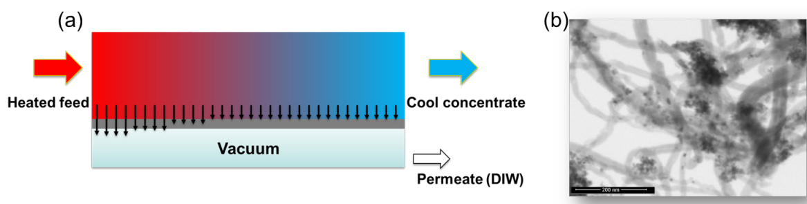
(a) Setup of the RF-heated MD system; (b) TEM images of the FE coated CNTs used for RF heating
