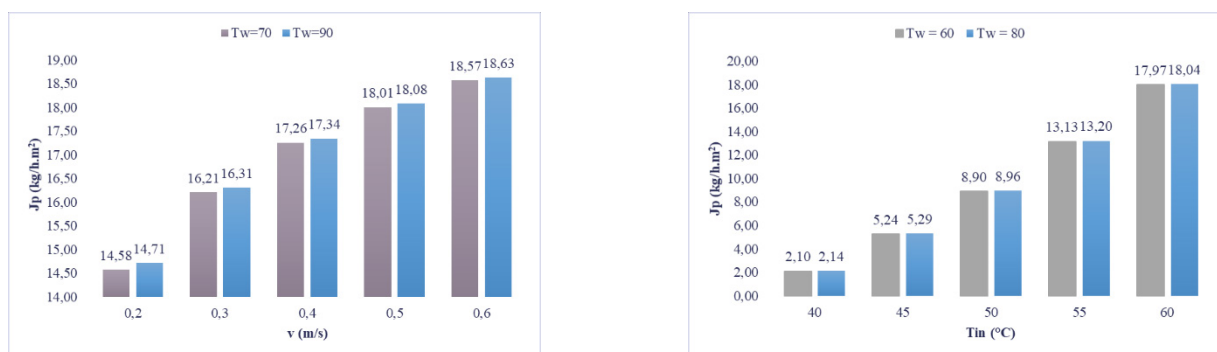
Fig. 2. Permeate flux (a) vs. fluid velocity for different T_{wall} at T_{in} = 60^\circ\text{C} (b) vs. T_{in} for different T_{wall} at v = 0.5 m/s.
