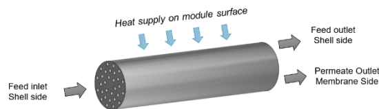
Fig. 1. SPC MD module geometry.
