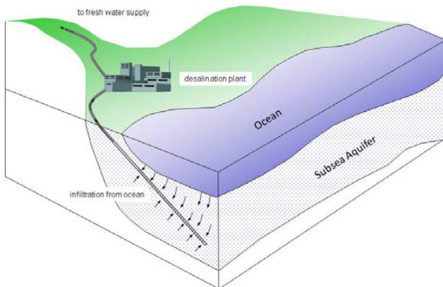
Fig. 1. Conceptual diagram of a slant well (from Williams [16]).
