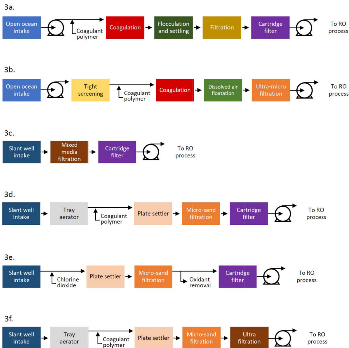
Fig. 3. Comparative process diagrams for the pretreatment of a conventional seawater desalination system using an open-ocean intake versus a slant well intake with differing water chemistry issues. Note that cartridge filters are not shown following the UF/MF filtration in scenarios because it is not logical to place a 45-micron filter after a 0.01-micron filter.
