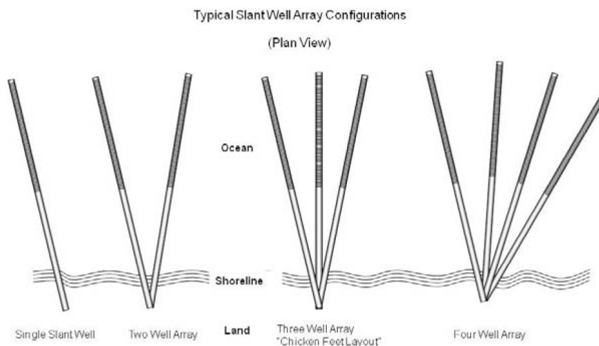
Fig. 2. Use of a one or more slant wells from a single near shore location (adapted from Williams [16]).
